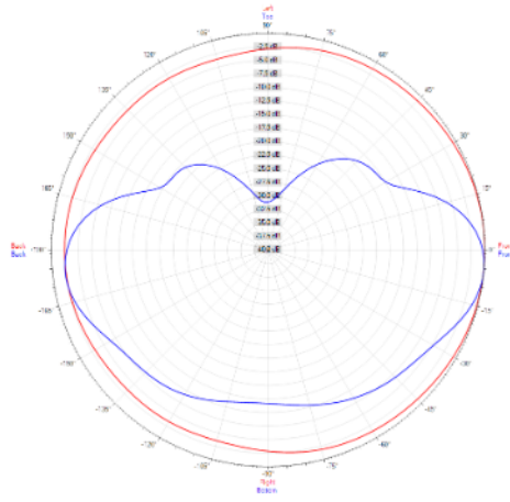
500 Hz 1/3 Oct
