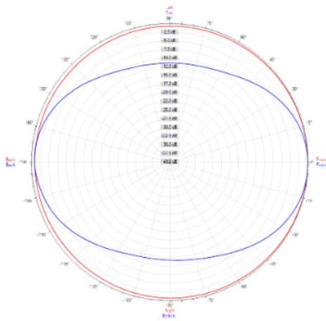
250 Hz 1/3 Oct
